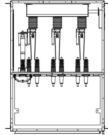
TOP VIEW (ROOF REMOVED)
