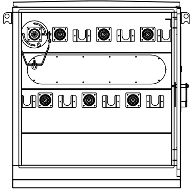
FRONT VIEW (DOOR REMOVED)
