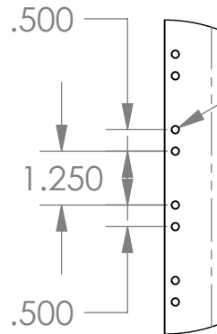
DETAIL A SCALE 1 : 4
